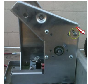
Remove Elevation Motor
